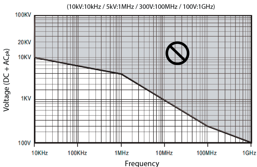
Figure 5: Voltage Derating Curve
