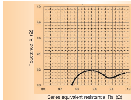
Frequency characteristics of a manganese battery (1 mHz to 100 kHz) [ cole-cole plot ]
